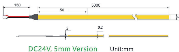
DC24V, 5mm Version Unit:mm
